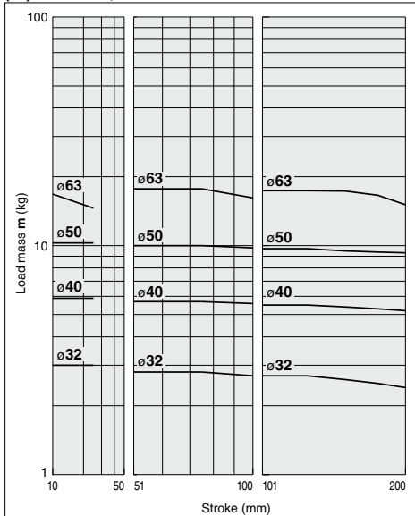
(27) L = 50 mm, V = 400 mm/s or less
