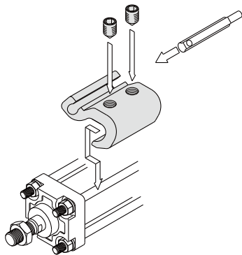
• Mounting example for D-M9□(V), M9□W(V), M9□A(V).
