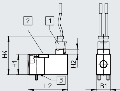
Plug connection on top
