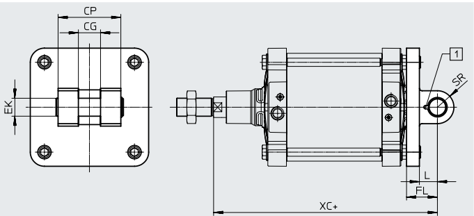
+ = plus stroke length [1] The pivot pin is secured against rotation with a spring pin.
