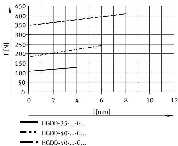
Spring force FF as a function of size and gripper jaw stroke l per gripper finger – with gripping force backup – HGDD-35 ... 50-...-G...
