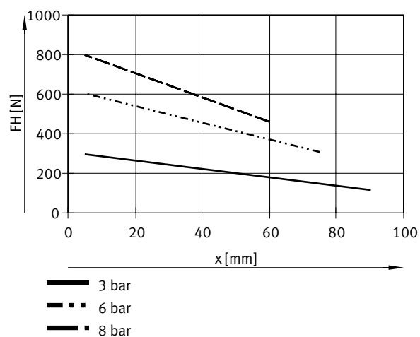
Gripping force FH per gripper jaw as a function of operating pressure and lever arm x – external gripping (closing), double-acting – HGDD-63
