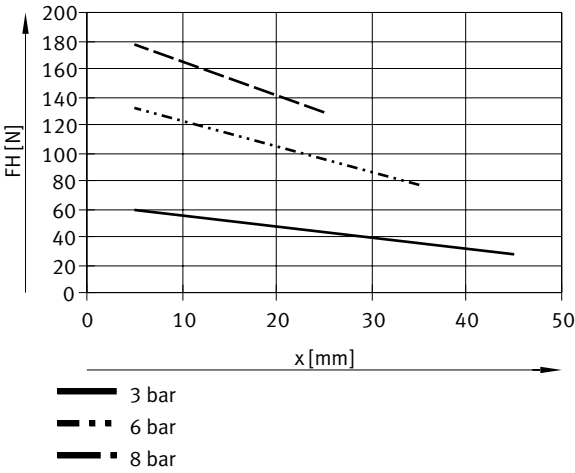
Gripping force FH per gripper jaw as a function of operating pressure and lever arm x – internal gripping (opening), double-acting – HGDD-35
