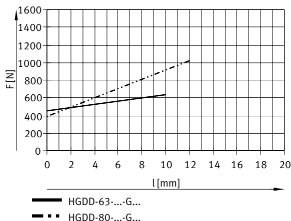
Spring force FF as a function of size and gripper jaw stroke l per gripper finger – with gripping force backup – HGDD-63 ... 80-...-G...
