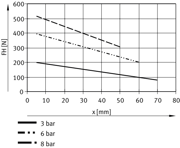
Gripping force FH per gripper jaw as a function of operating pressure and lever arm x – internal gripping (opening), double-acting – HGDD-50
