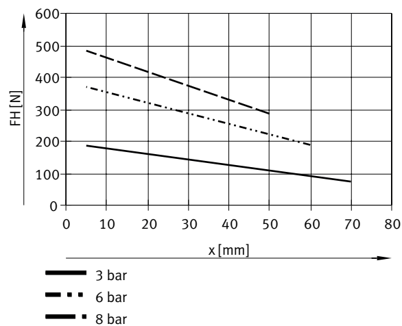
Gripping force FH per gripper jaw as a function of operating pressure and lever arm x – external gripping (closing), double-acting – HGDD-50
