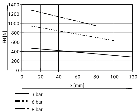
Gripping force F_H per gripper jaw as a function of operating pressure and lever arm x – internal gripping (opening), double-acting – HGDD-80
