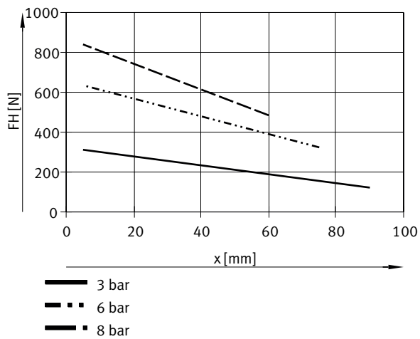
Gripping force F_H per gripper jaw as a function of operating pressure and lever arm x – internal gripping (opening), double-acting – HGDD-63
