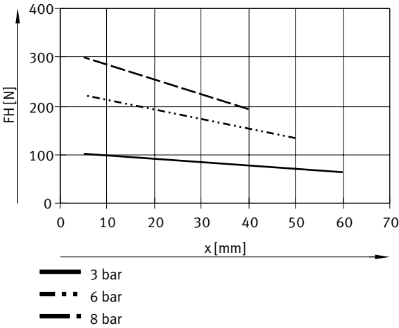
Gripping force FH per gripper jaw as a function of operating pressure and lever arm x – internal gripping (opening), double-acting – HGDD-40
