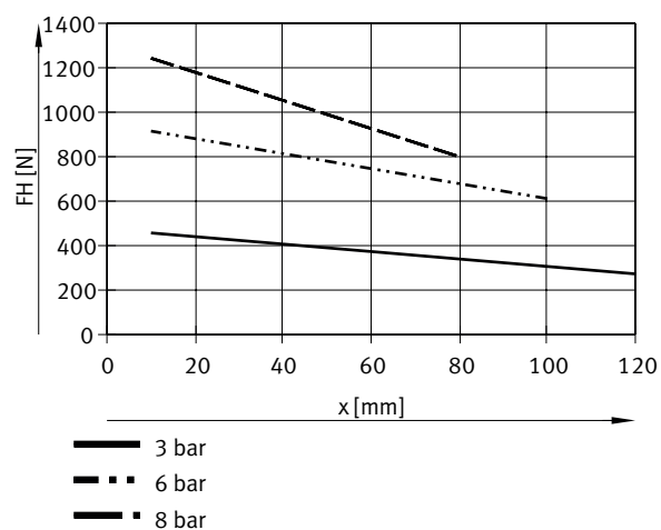
Gripping force FH per gripper jaw as a function of operating pressure and lever arm x – external gripping (closing), double-acting – HGDD-80
