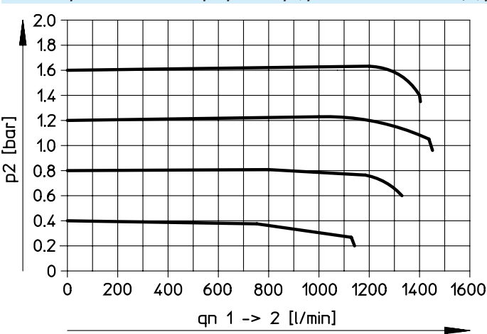
Flow rate q_n as a function of output pressure p_2 , pneumatic connection G1/4, pressure regulation range 0... 2 bar
