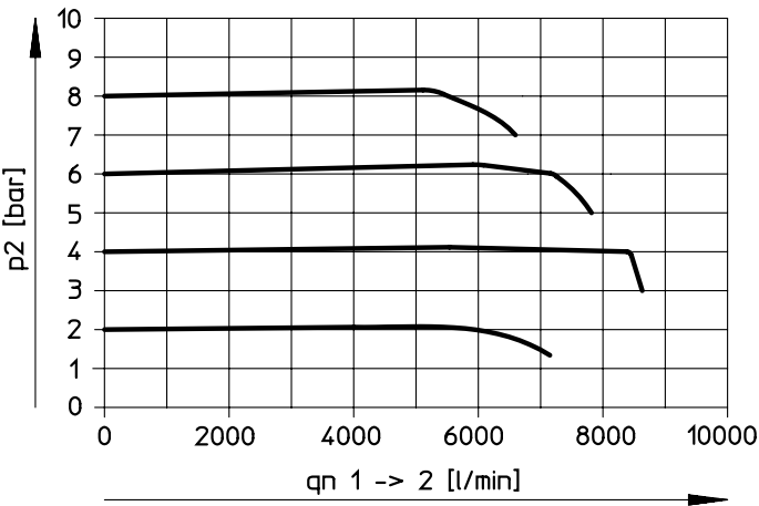
Flow rate q_n as a function of output pressure p_2 , pneumatic connection G1/2, pressure regulation range 0... 10 bar
