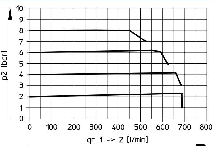
Flow rate q_n as a function of output pressure p_2 , pneumatic connection G1/8, pressure regulation range 0... 10 bar
