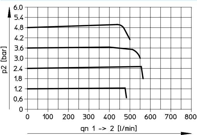
Flow rate q_n as a function of output pressure p_2 , pneumatic connection G1/8, pressure regulation range 0... 6 bar
