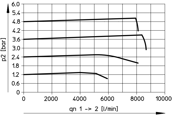
Flow rate q_n as a function of output pressure p_2 , pneumatic connection G1/2, pressure regulation range 0... 6 bar
