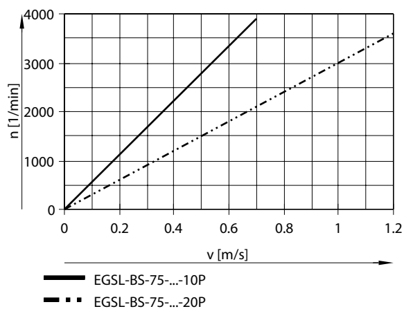
Rotational speed n as a function of feed speed v for size 75
