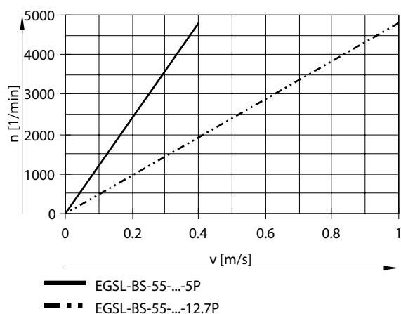
Rotational speed n as a function of feed speed v for size 55
