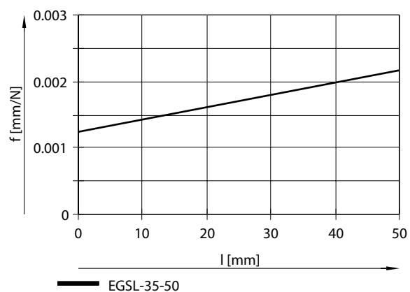
Deflection x as a function of force F_y for size 35
