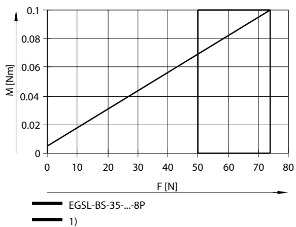
Drive torque M as a function of feed force F for size 35
