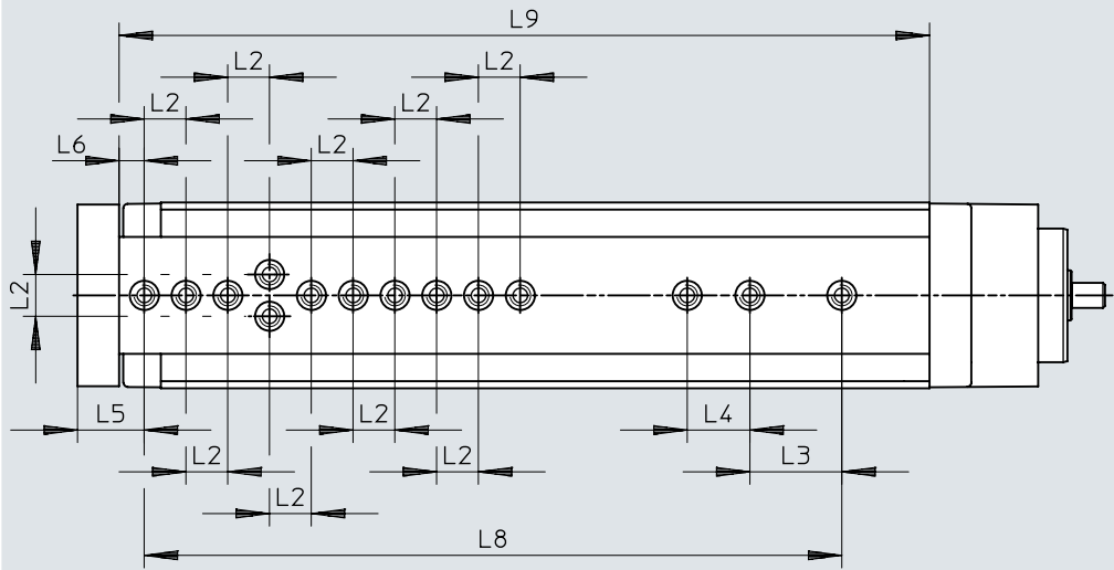
Dimensions – EGSL-45-100
