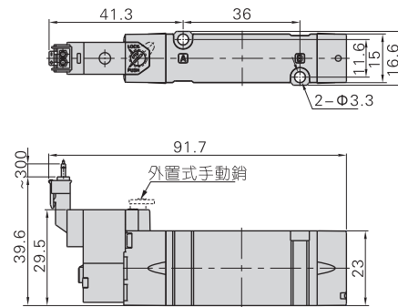
7MV110(先導閥M型)
