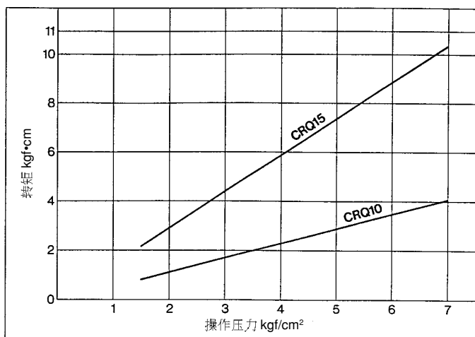
CRQBW10·15
