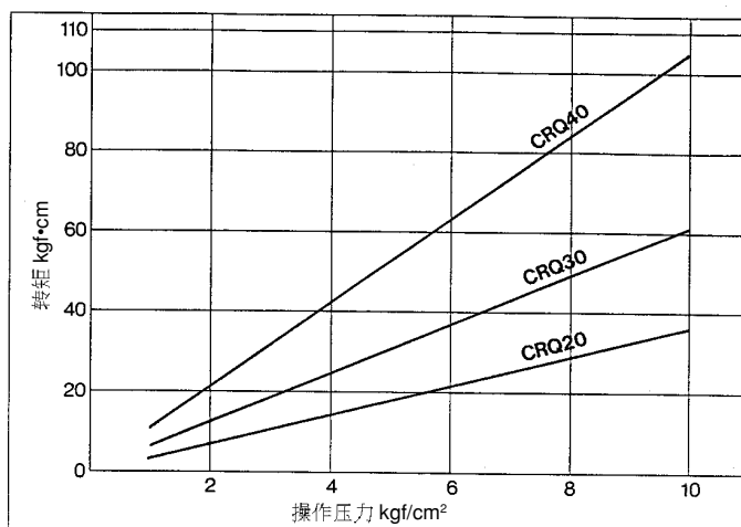
CRQBW20·30·40
