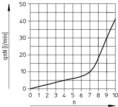
Standard nominal flow rate q_{nN} at 6 \rightarrow 5 bar as a function of turns of the adjusting screw n GRLA/GRLZ/GRGA/GRGZ-M3
