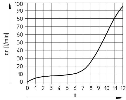
Standard flow rate q_n at 6 \rightarrow 0 bar as a function of turns of the adjusting screw n GRLA/GRLZ/GRGA/GRGZ-M3
