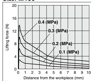
Size: \square 150
