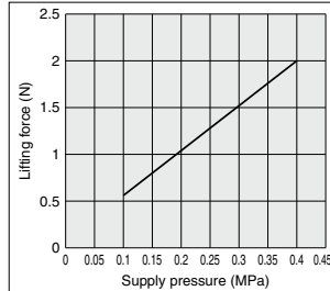
Size: \phi 25
