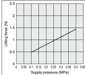
Size: \phi 20
