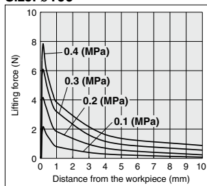
Size: \phi 100
