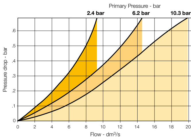
Flow Characteristics - 1/4 Inch Ports 04L00G*
