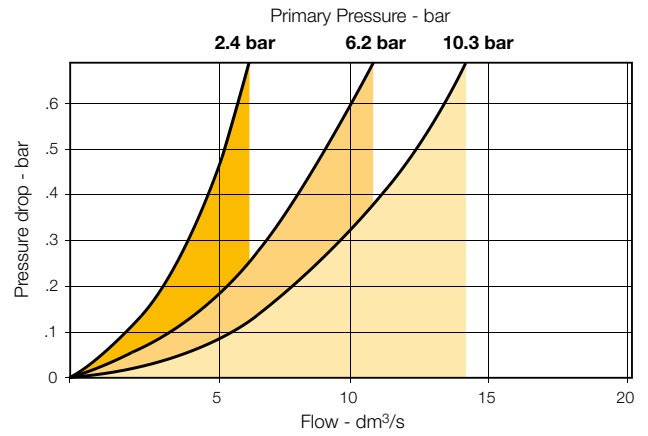
Flow Characteristics - 1/4 Inch Ports 10F11E*
